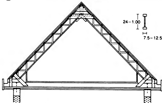
3 Couple close roof in timber framing with lifetime guaranteed glued joints with 45^\circ inclined struts as twinned supports over span < 25\text{m}
